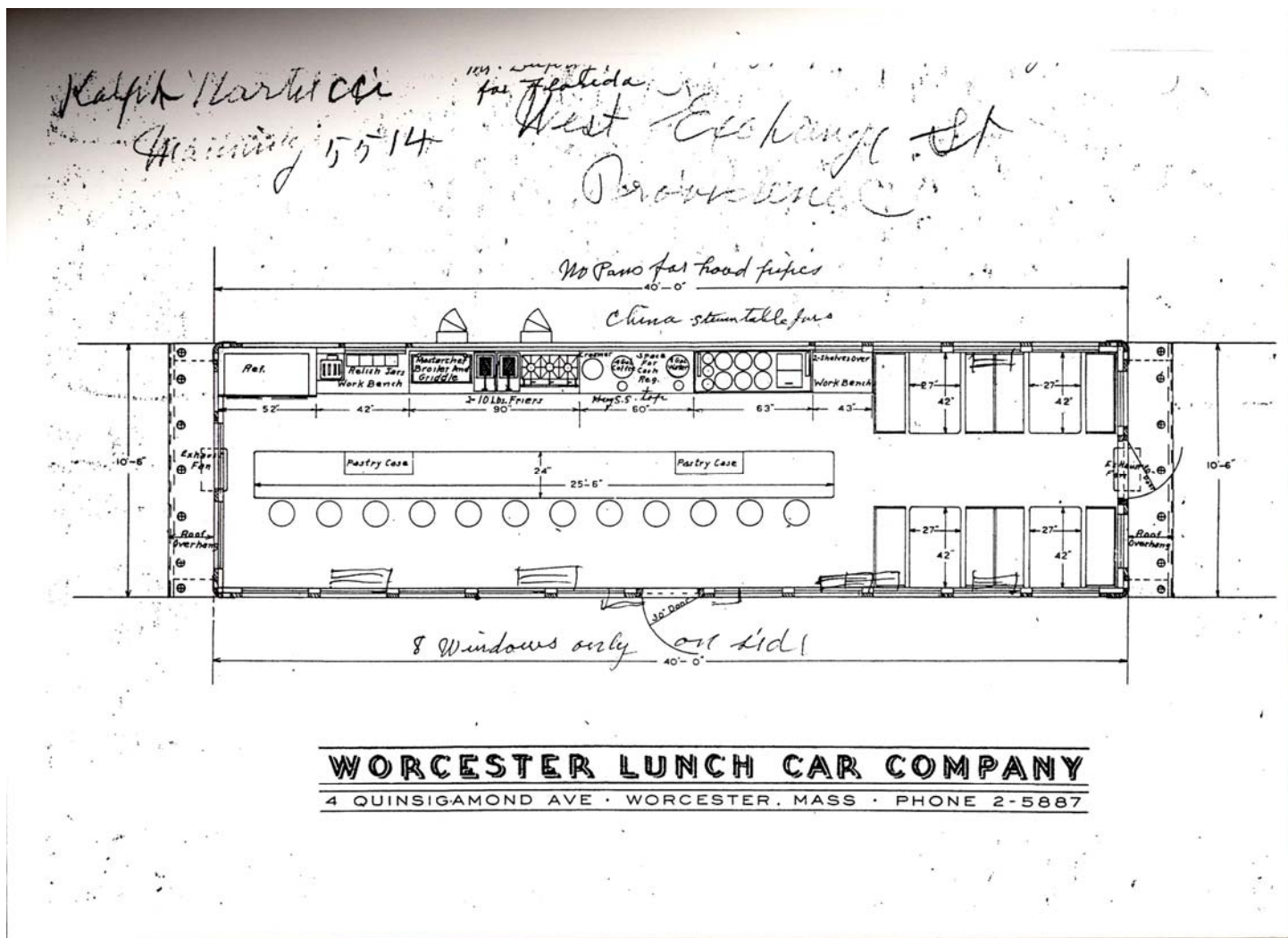
Drawing 1: [Car #806], ca. 1947 in Worcester Lunch Car Company, "Layout Sketches," ca 1920s-1957. Copies courtesy of Kim Smith, Moosup, CT.
